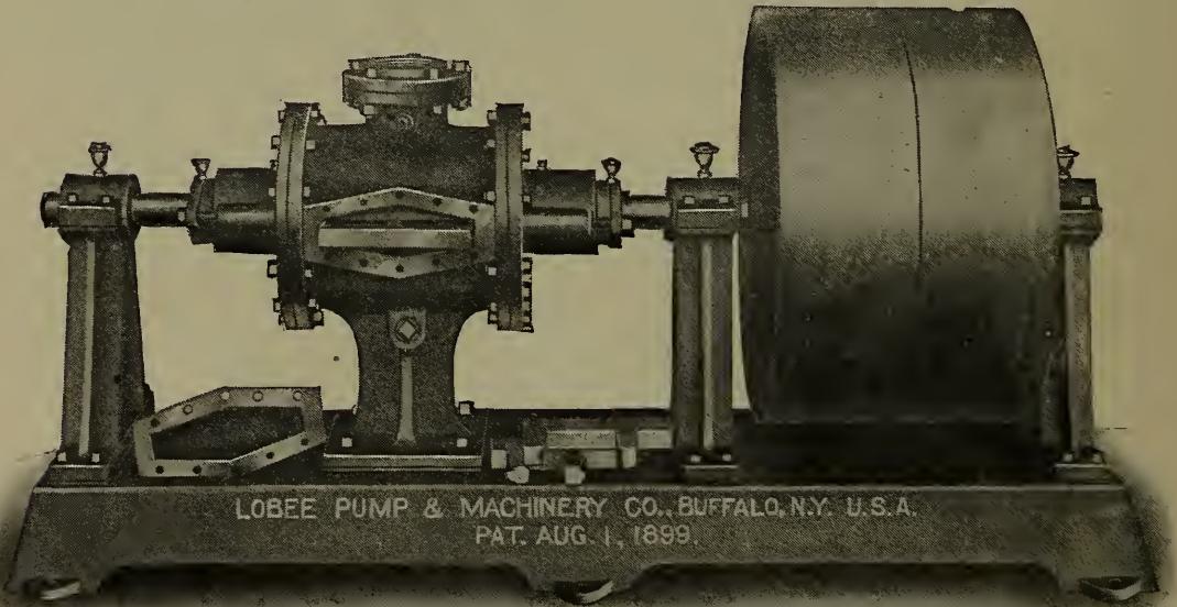
SPECIAL NO. 6 MOTOR PUMP For Pumping Lye, Soap, Oils, etc.
